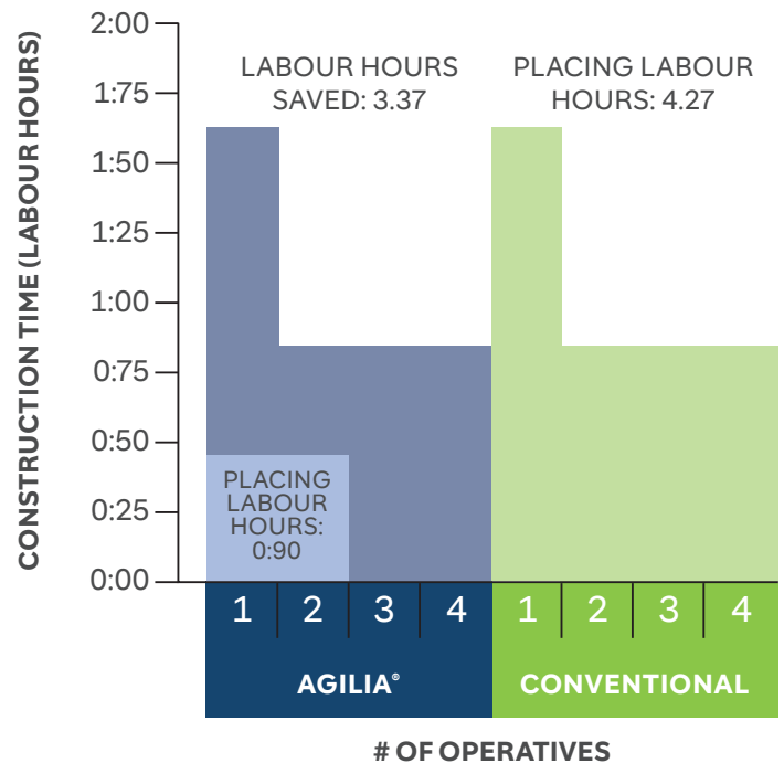
Placement* time of 1m 2 concrete
