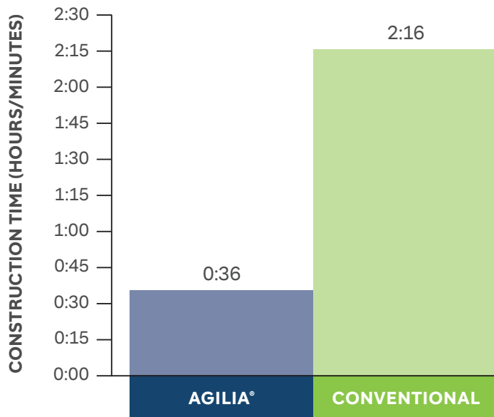
Placement* time of 1m 2 concrete
